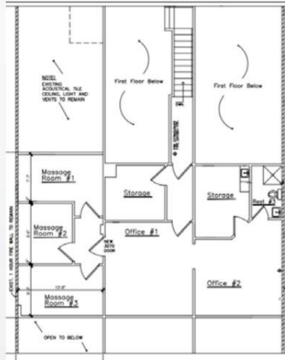
SECOND FLOOR 1,494 SF
